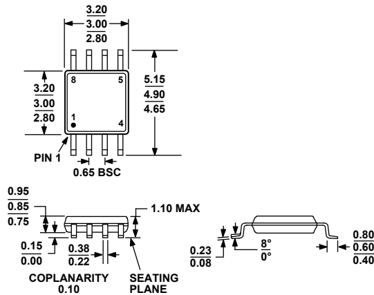
COMPLIANT TO JEDEC STANDARDS MO-187-AA Figure 57. 8-Lead Mini Small Outline Package [MSOP] (RM-8) Dimensions shown in millimeters
