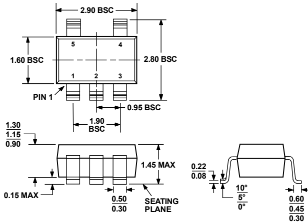
COMPLIANT TO JEDEC STANDARDS MO-178-AA Figure 55. 5-Lead Small Outline Transistor Package [SOT-23] (RJ-5) Dimensions shown in millimeters
